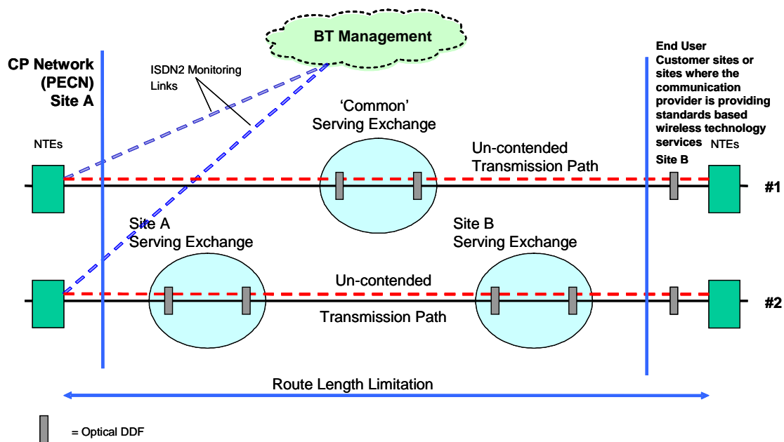
Figure 1. WES 622 service configurations
