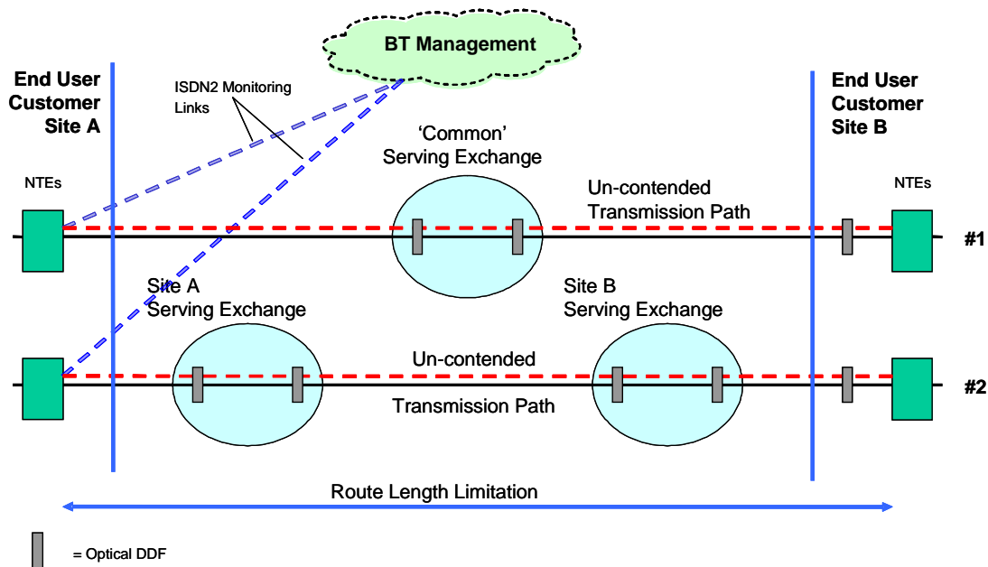
Figure 2. WEES 155 service configuration
