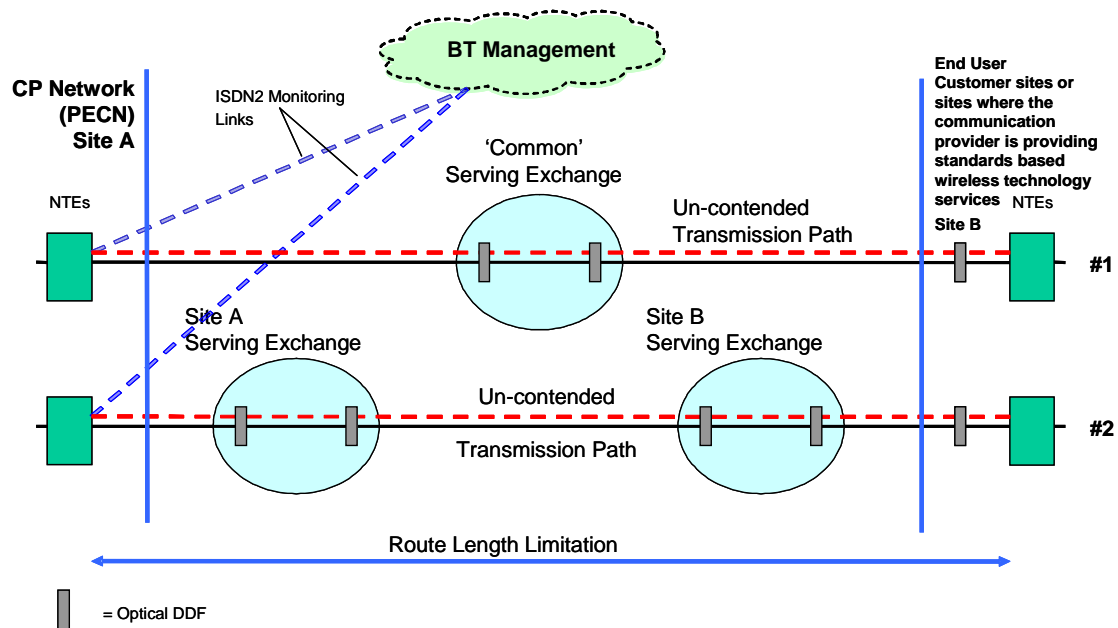
Figure 1 WES 155 service configuration
