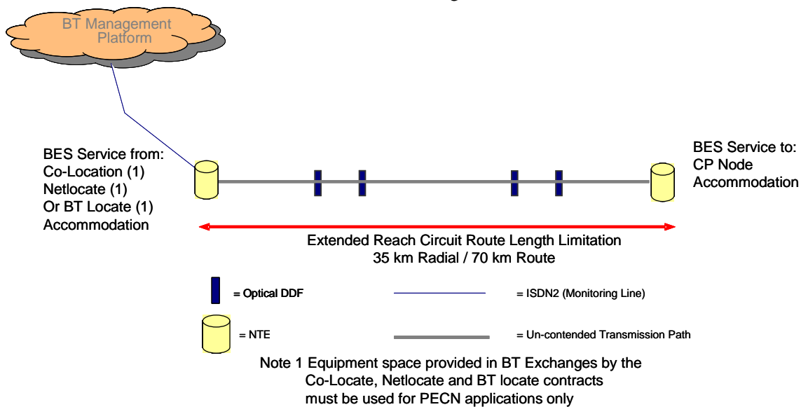
Figure 2. Typical BES 1000ER service configuration
