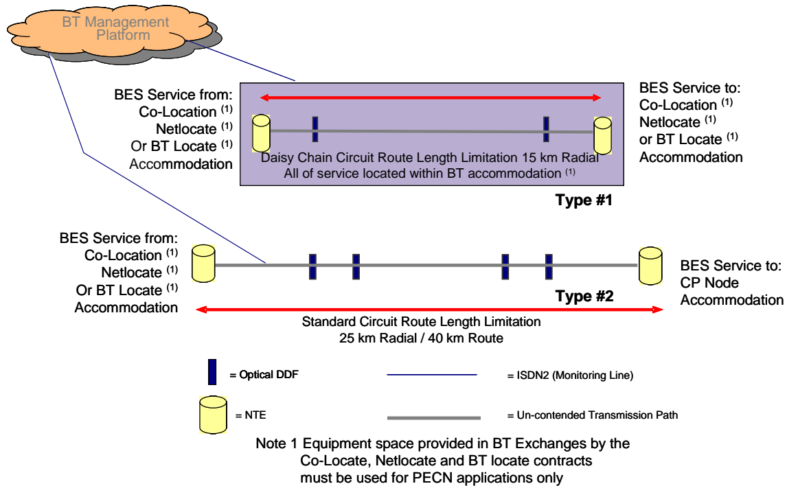
Figure 1. Typical BES 1000 service configurations
