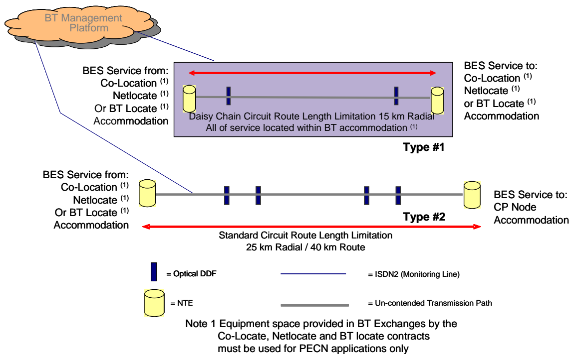
Figure 1. BES 10 Service Configuration
