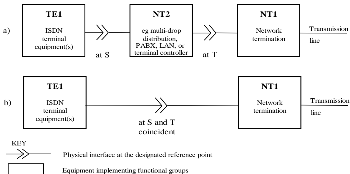
Figure A.1 - Examples of user configurations
